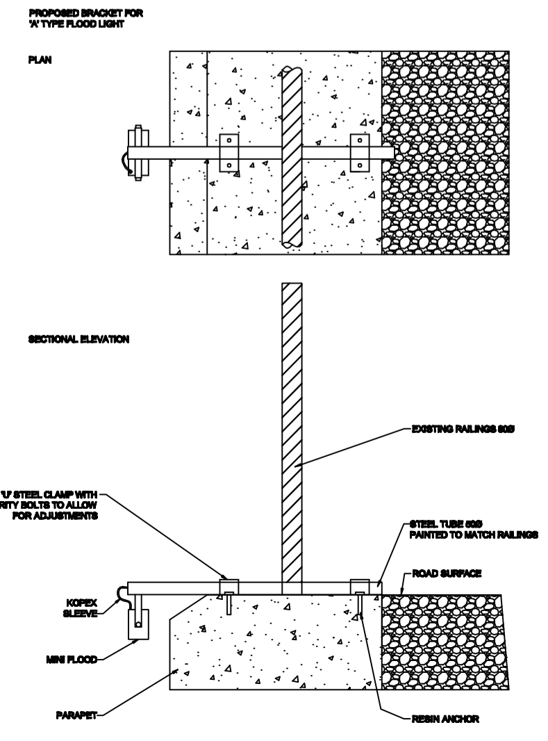
LUMINAIRE TYPE 'A' LED FLOOD TO WASH LIGHT DOWN PIER 1:20 @ A1
