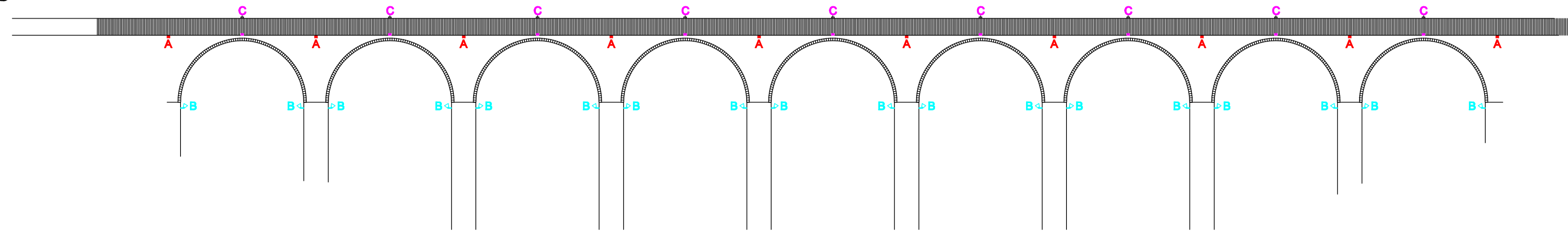
VIADUCT ELEVATION 1:200 @ A1
