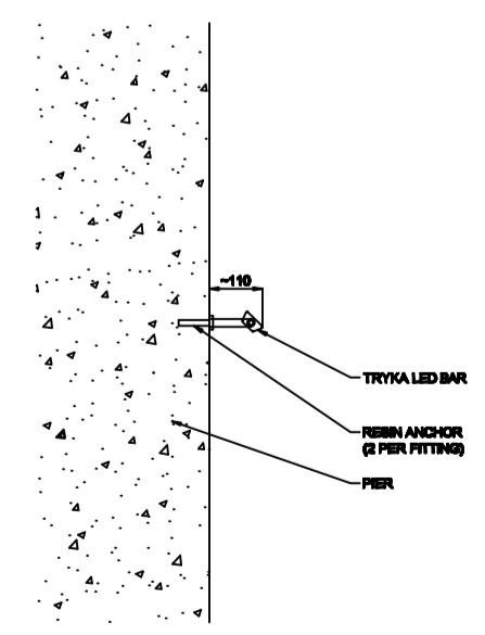
LUMINAIRE TYPE 'B' LED BAR TO WASH UNDERSIDE OF ARCH 1:20 @ A1
