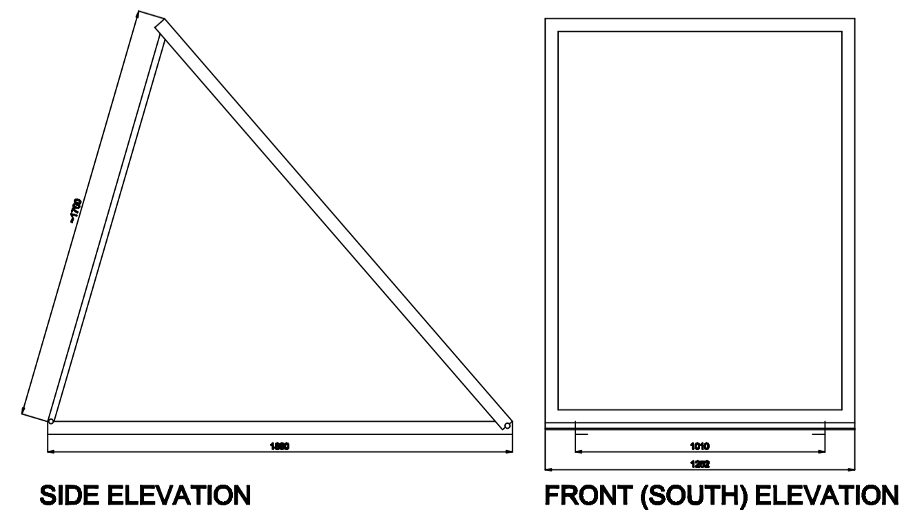
PHOTOVOLTAIC CELLS (4 off) 1:20 @ A1
