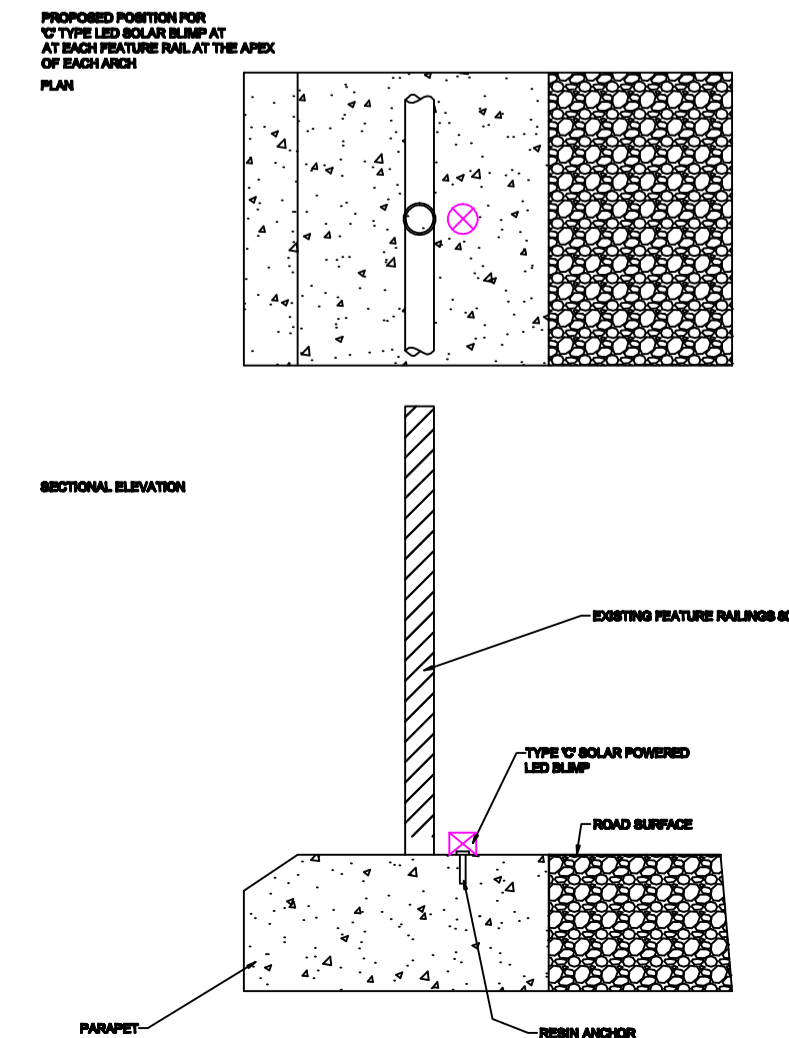
LUMINAIRE TYPE 'C' SOLAR POWERED LED BLIMP UPLIGHT 1:20 @ A1
